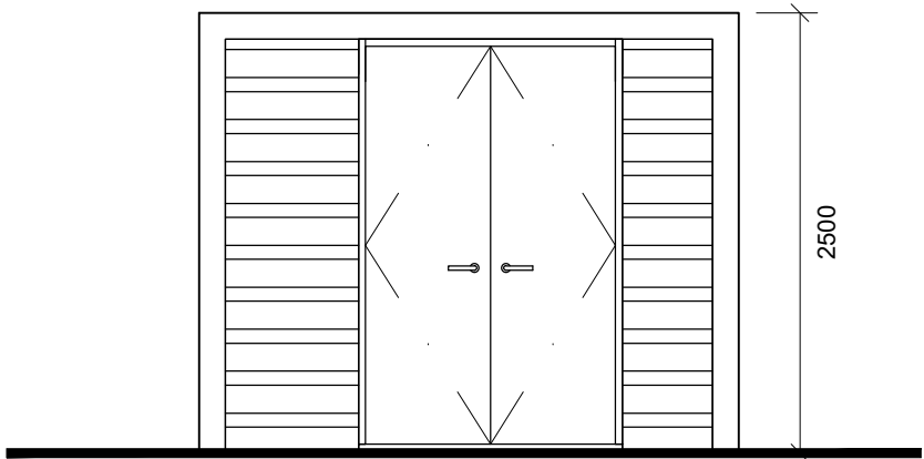
2 EAST ELEVATION 1:50
