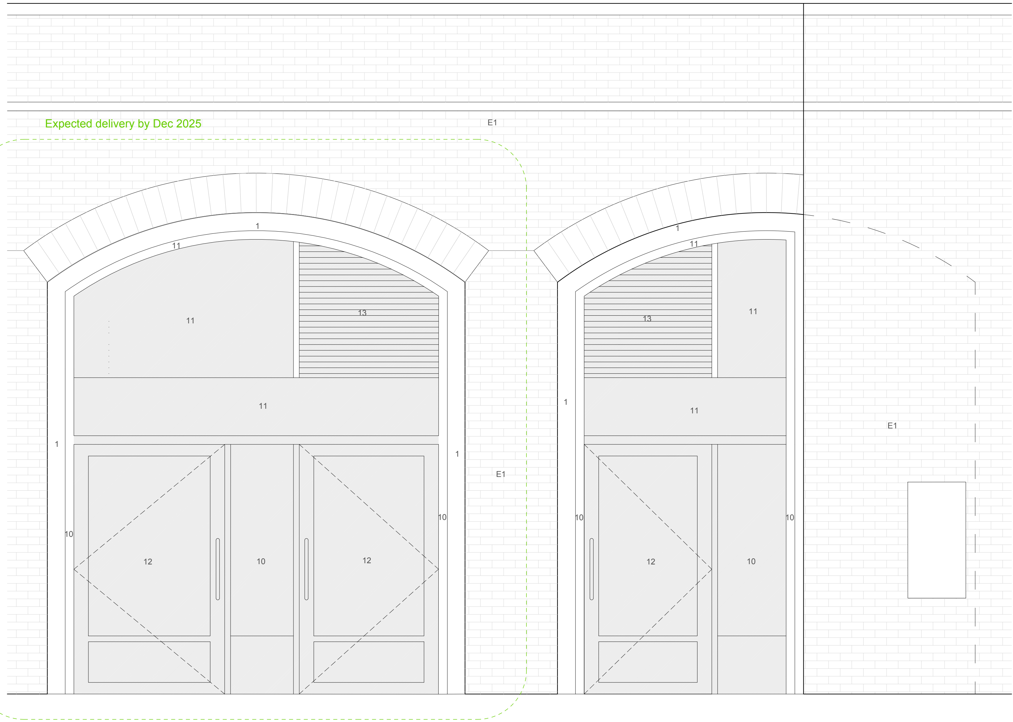
01 Proposed service facade elevation 1:20 @ A1
