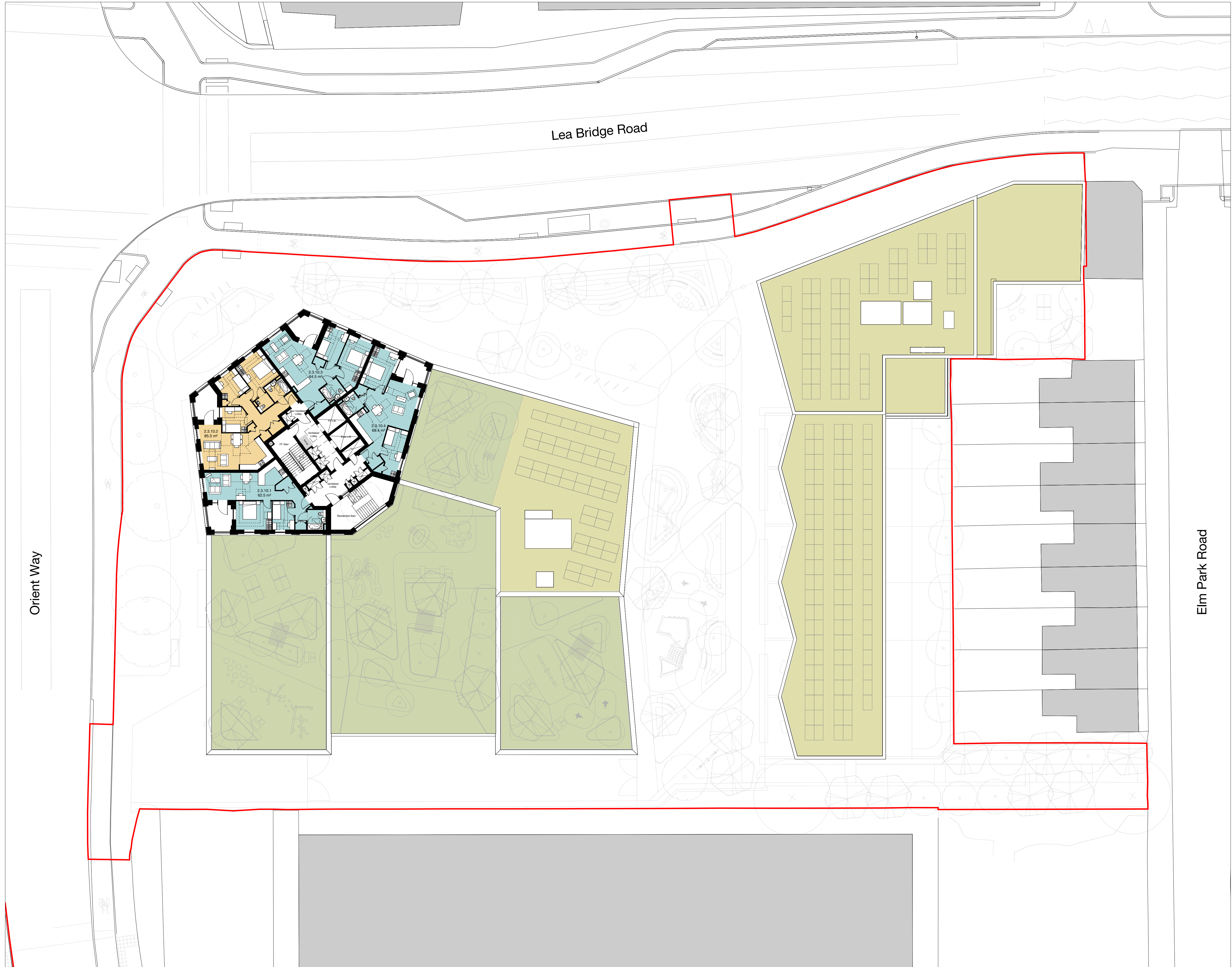
1 Site 2 - Proposed Tenth Floor Plan 1 : 200
