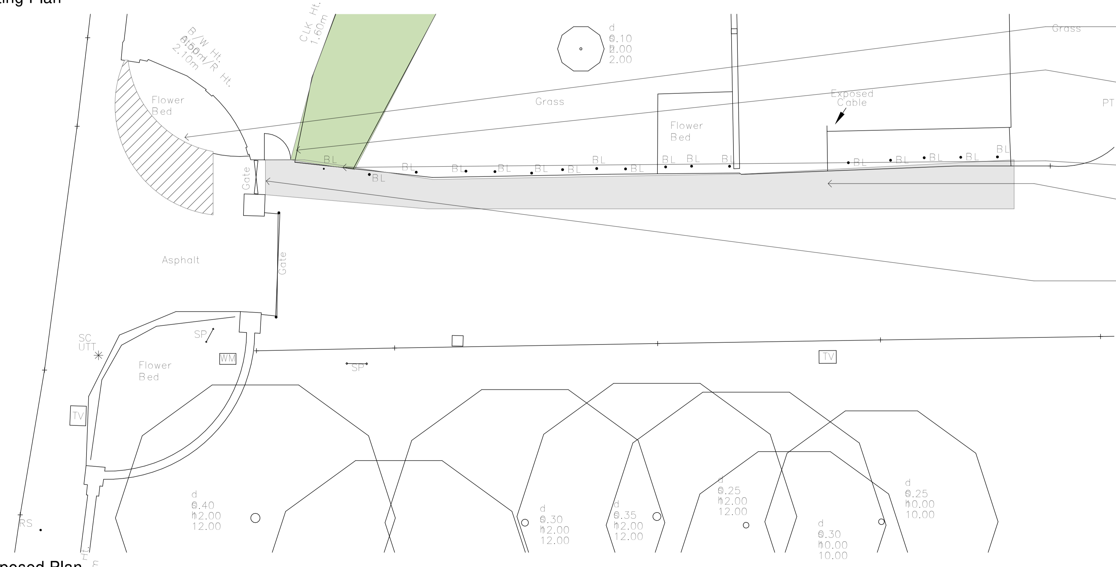
Proposed Plan
