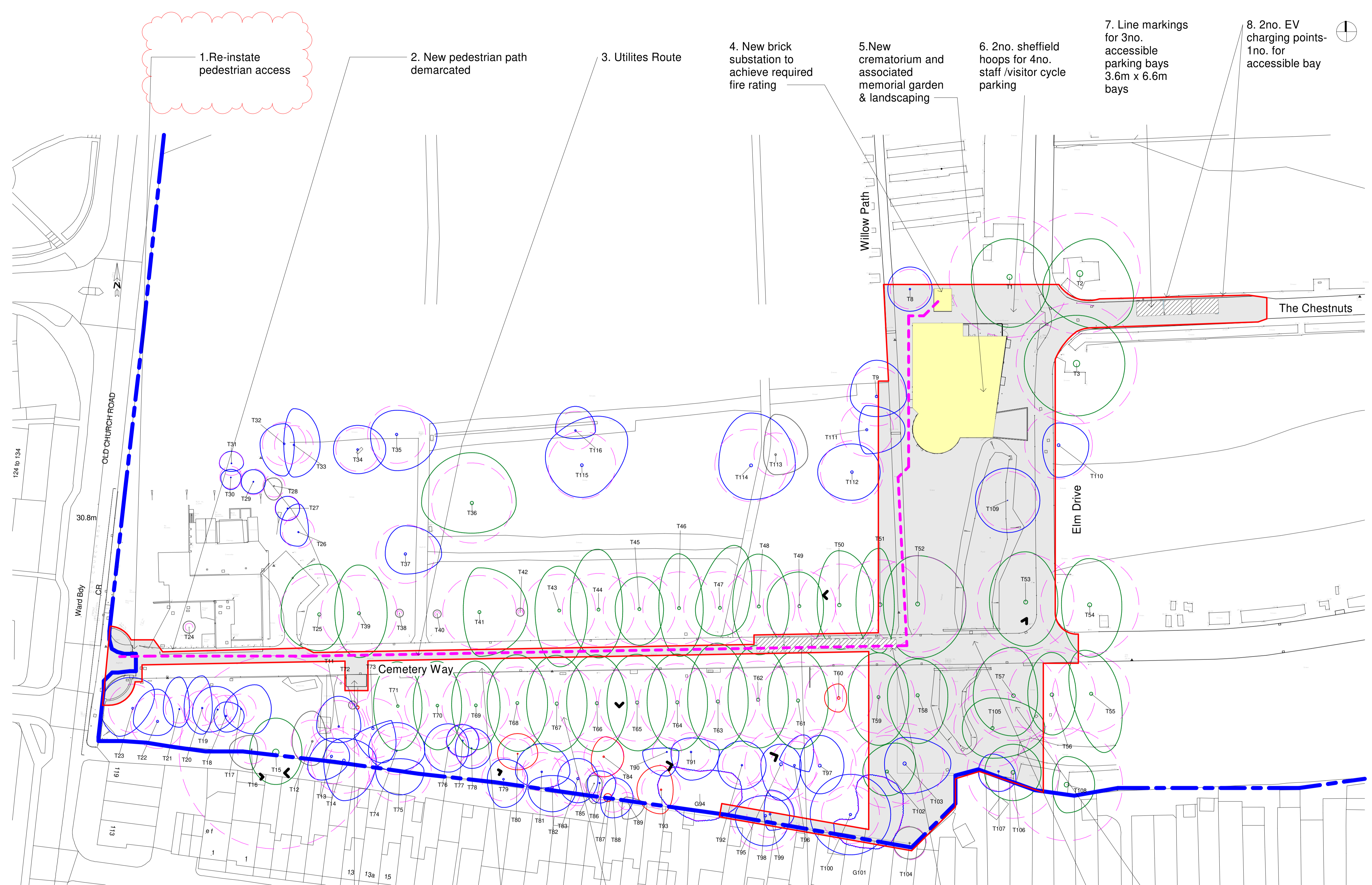
Proposed Site Plan 1 to 500 1:500
