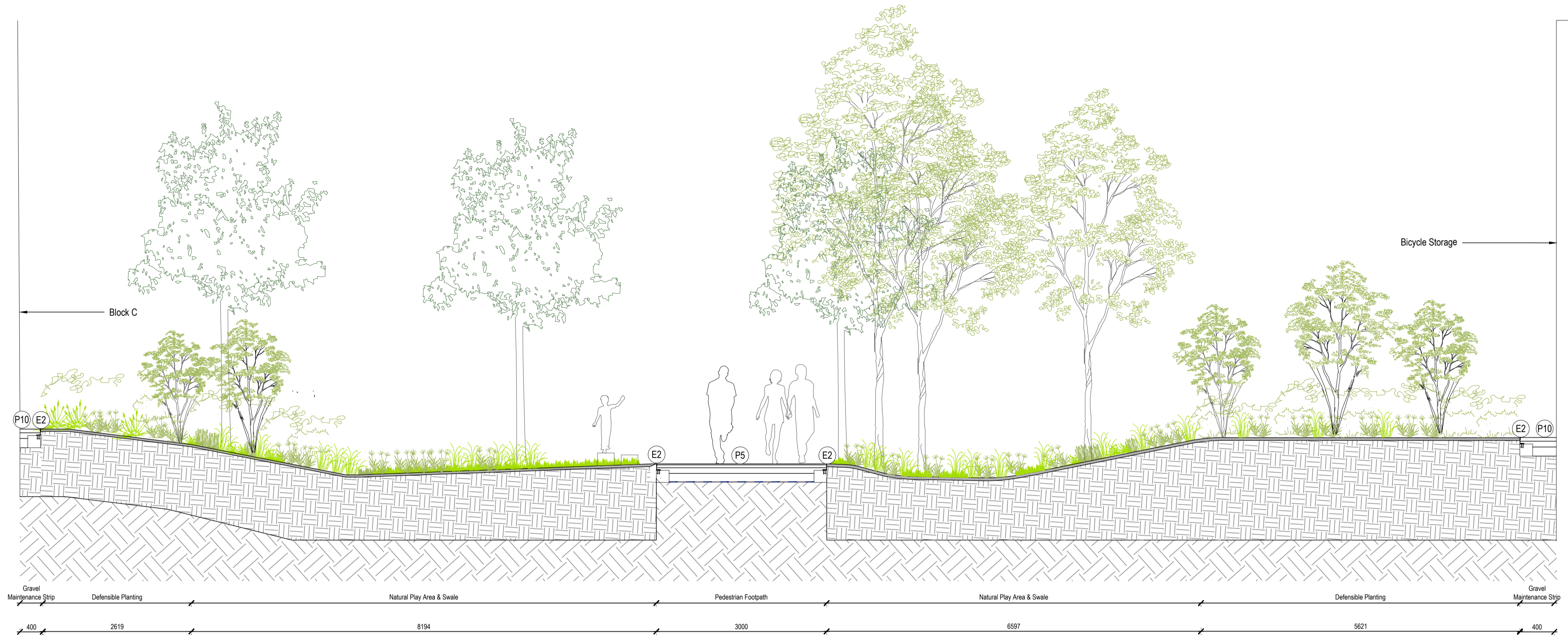
01 Lower Valley - Landscape Section C Scale 1:50@A1
