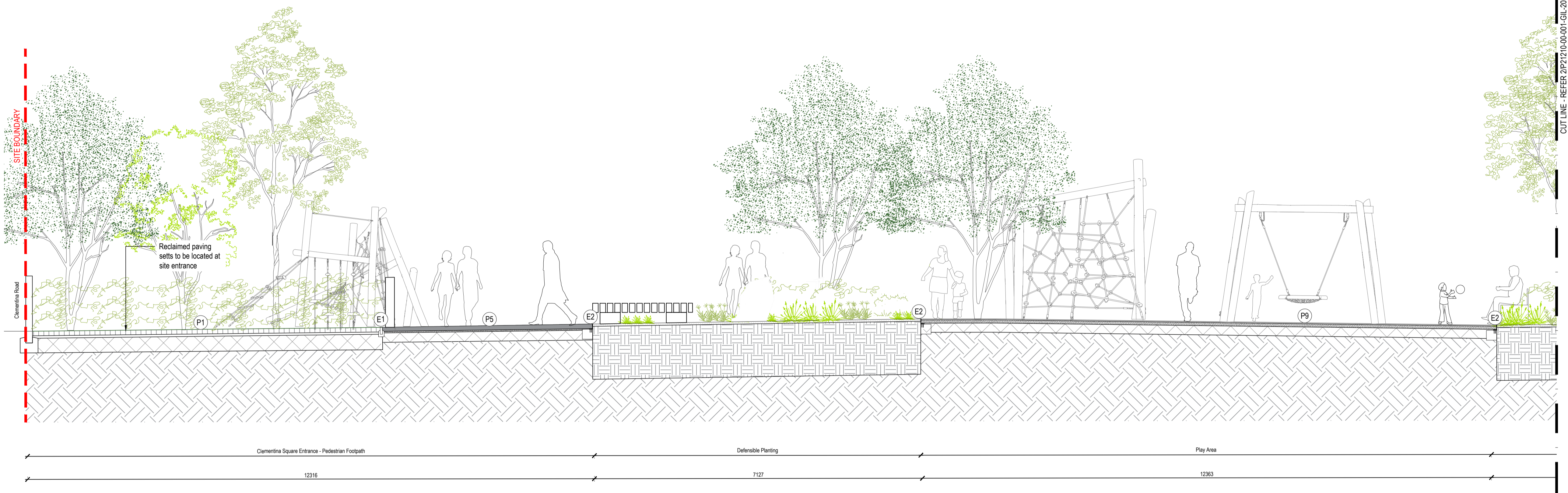
01 200 Clemantina Square - Landscape Section A Scale 1: 50@A1
