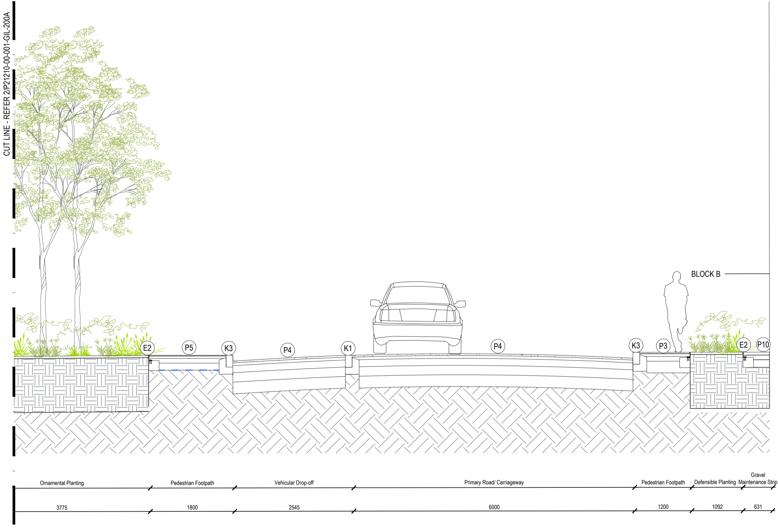
02 200 Clemantina Square - Landscape Section A (Continued) Scale 1: 50@A1
