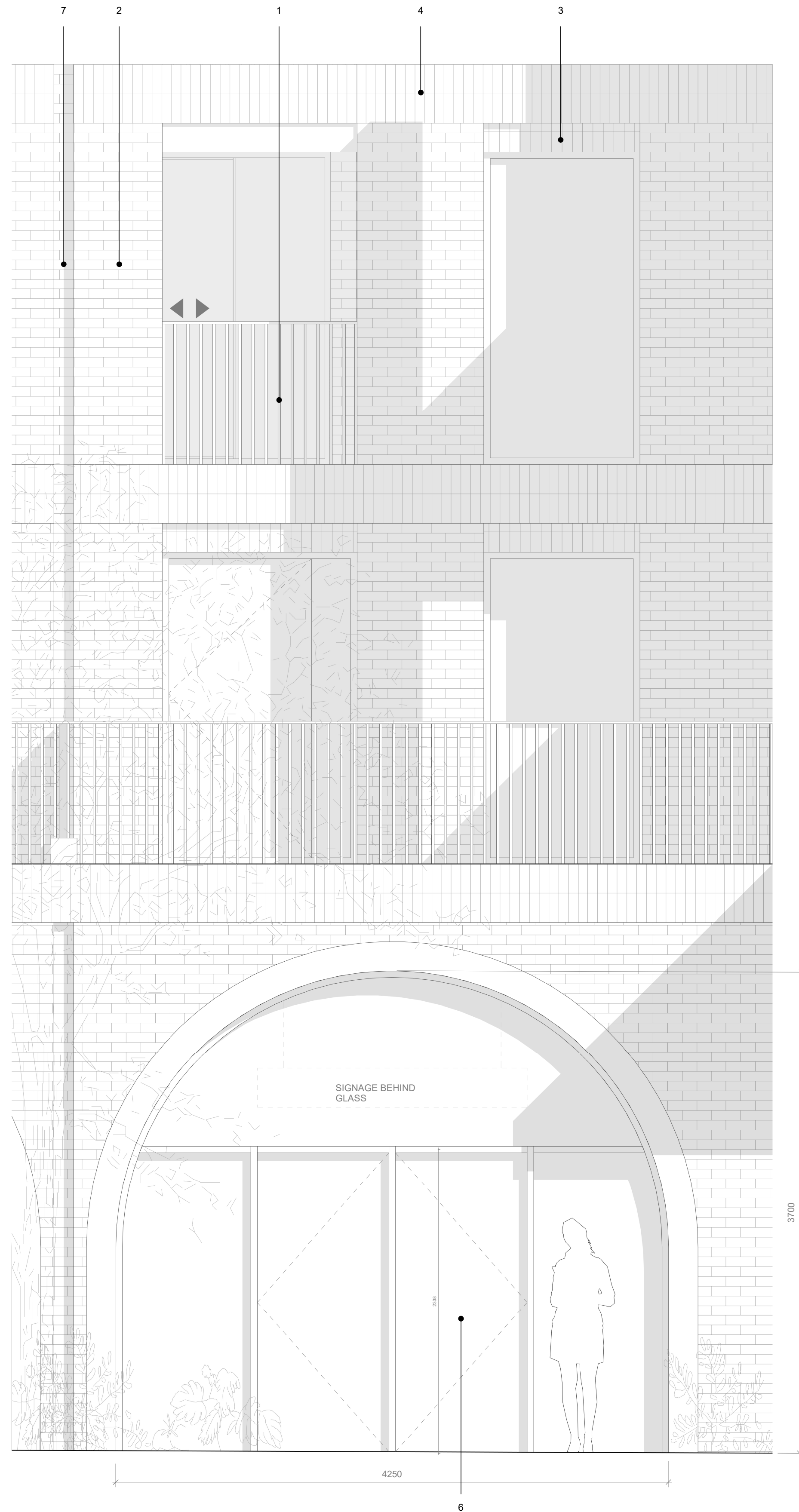
1 Proposed Commercial Arch Elevation Study 1 : 25
