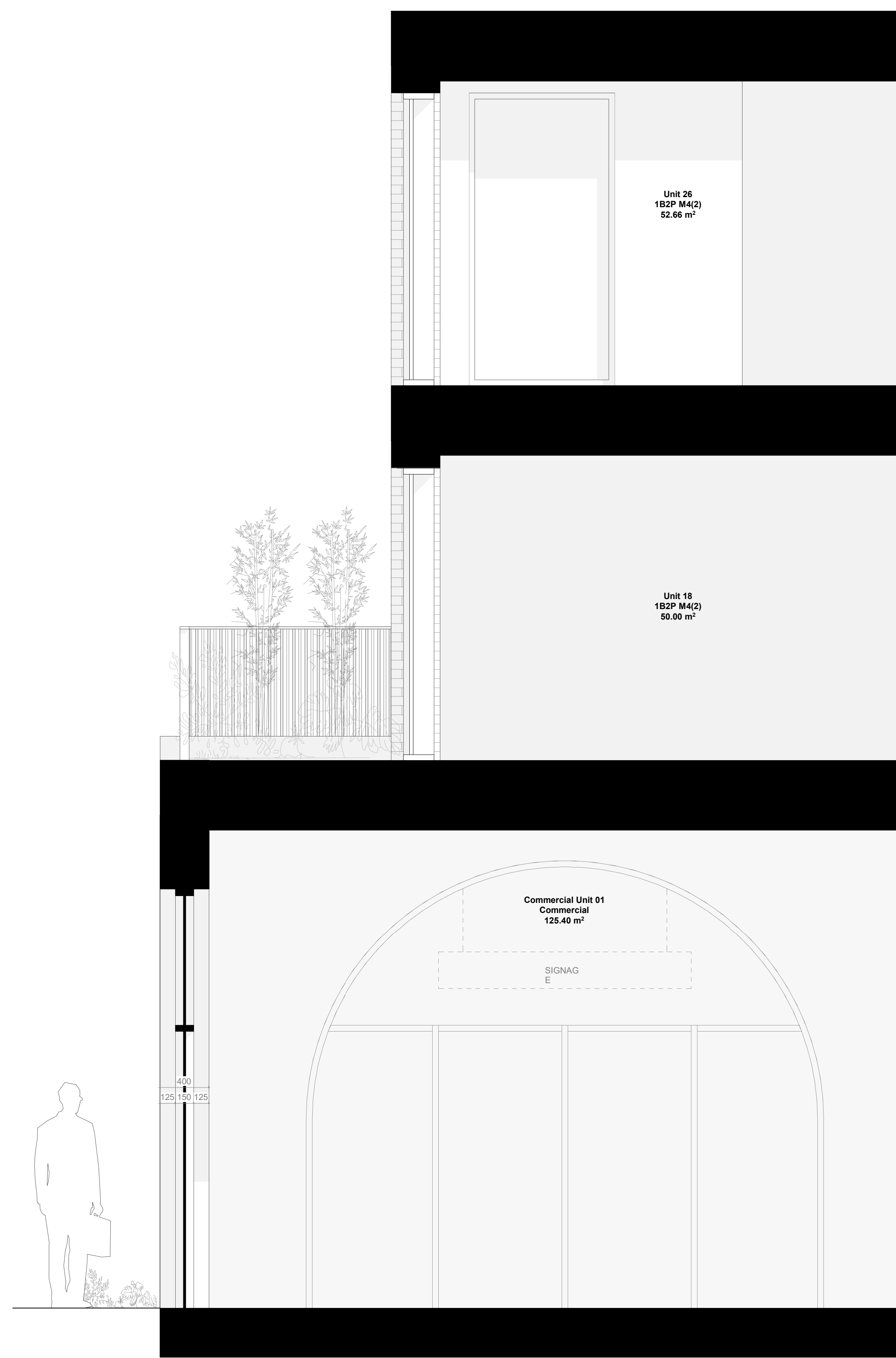
2 Proposed Commercial Arch Section 1 : 25
