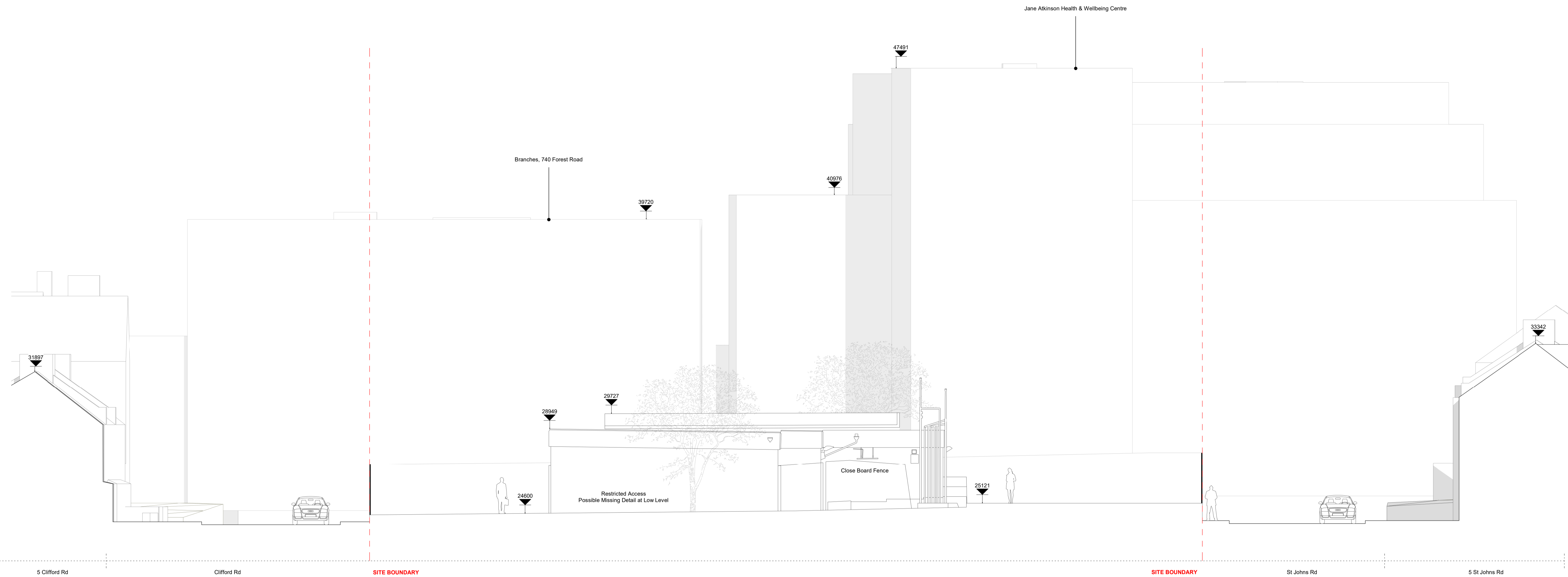
Existing North Elevation 1 : 100
