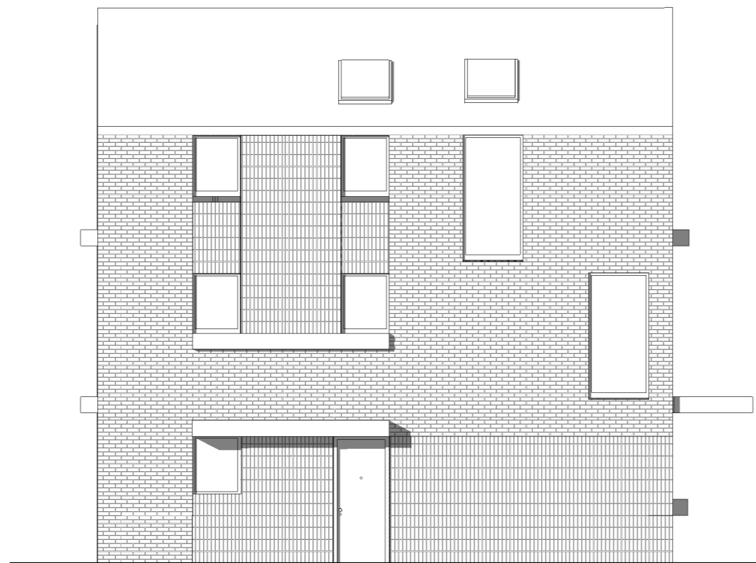
East Elevation Building 2 1 : 100
