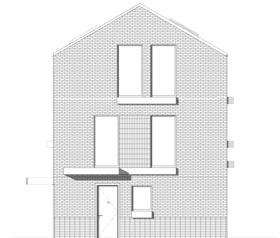
North Elevation Building 2 1 : 100
