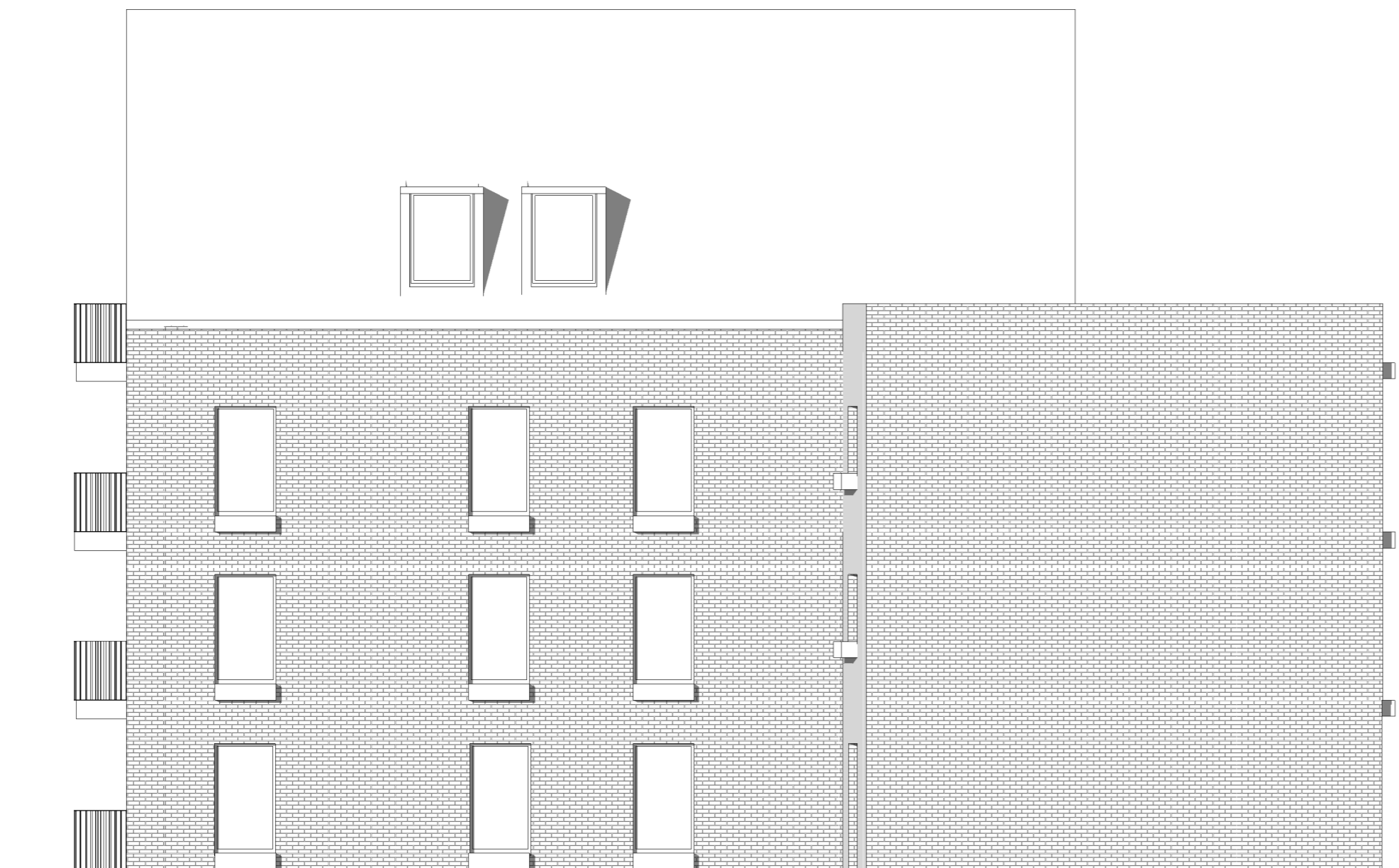
West Elevation Building 1 1 : 100
