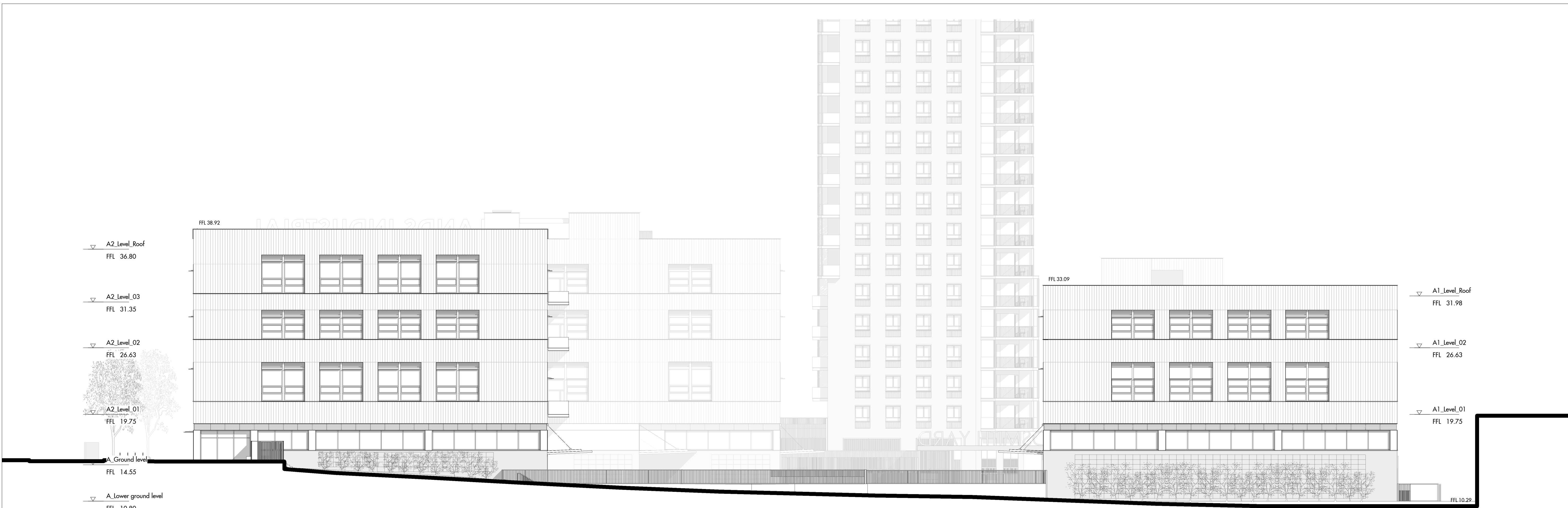
Boundary fence - North elevation
