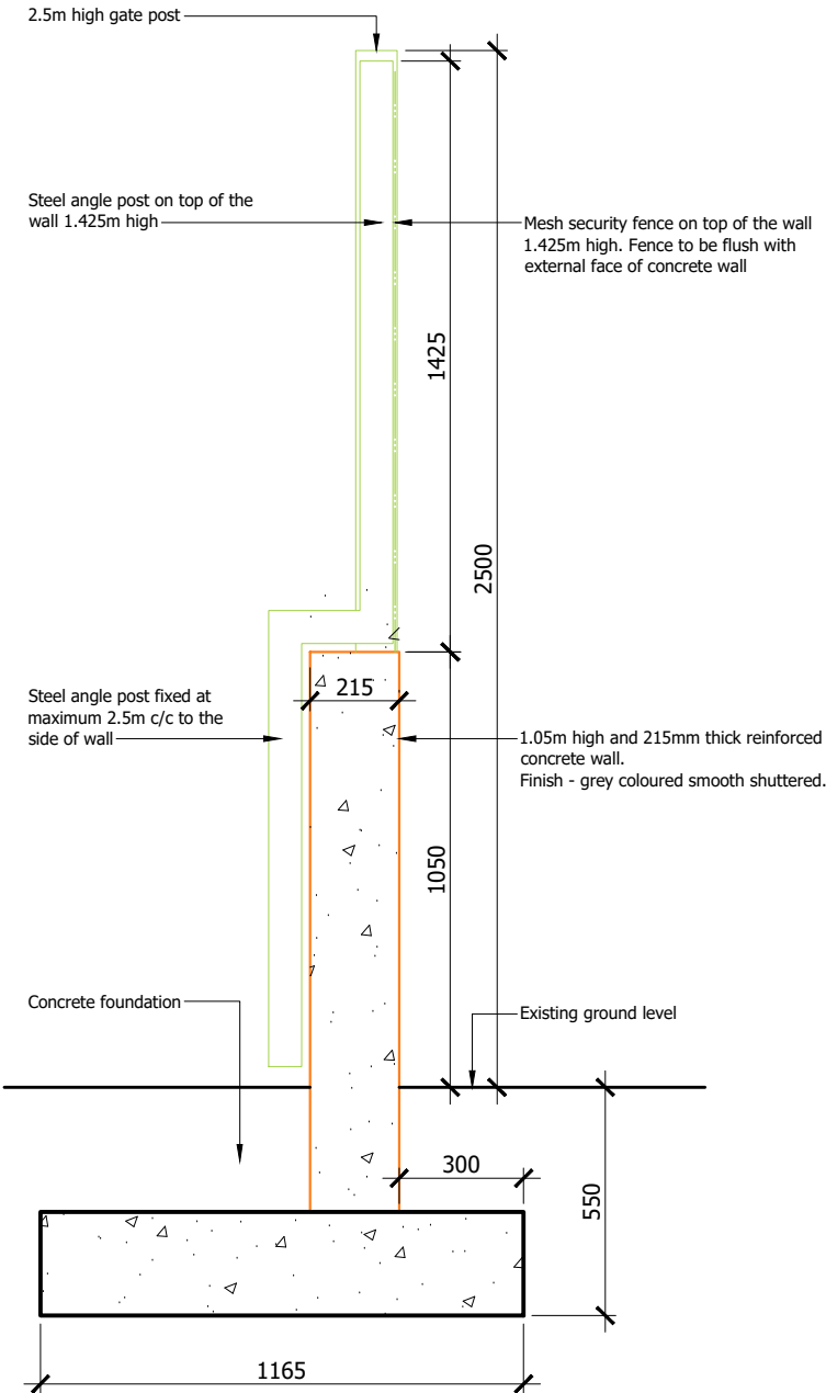
CROSS SECTION OF WALL WITH MESH FENCE OVER
