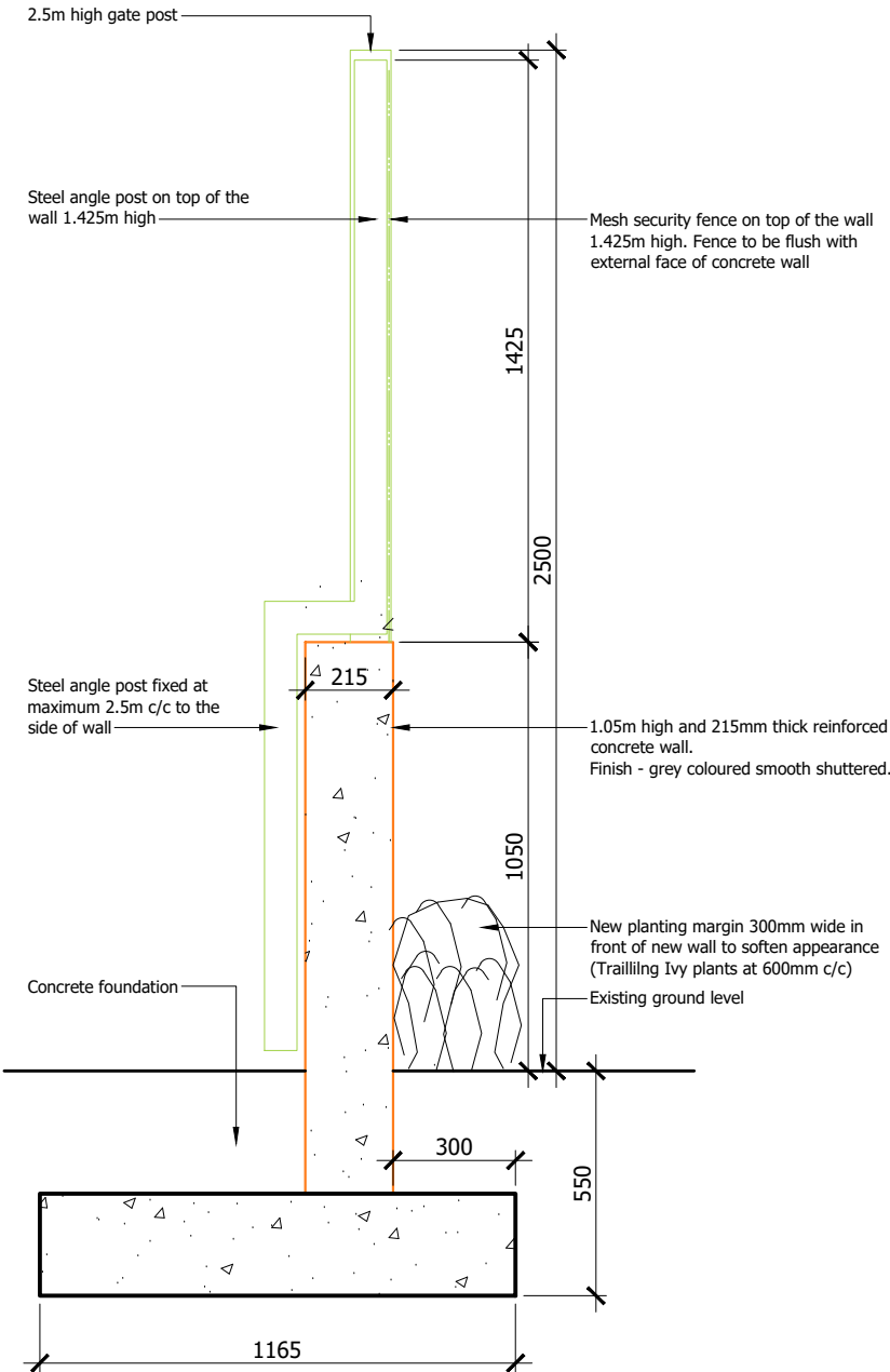
CROSS SECTION OF WALL WITH MESH FENCE OVER
