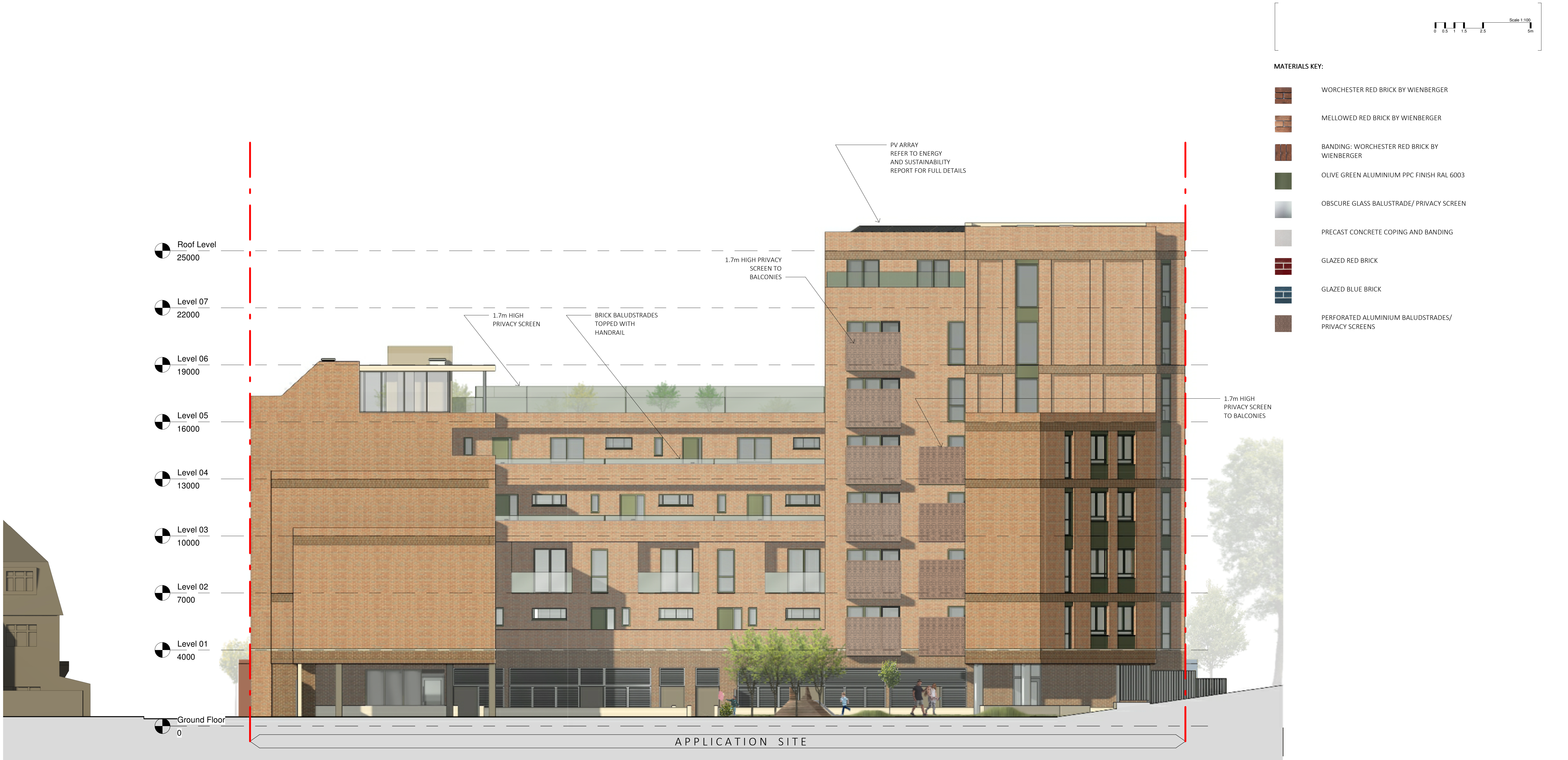
1 South Elevation Scale: 1 : 100
