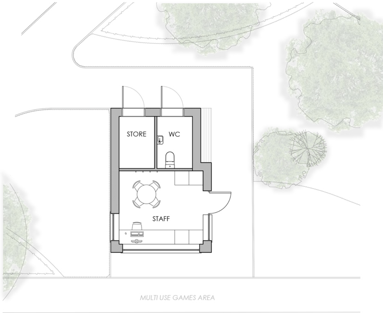
Proposed Floor Plan Staff Hut
