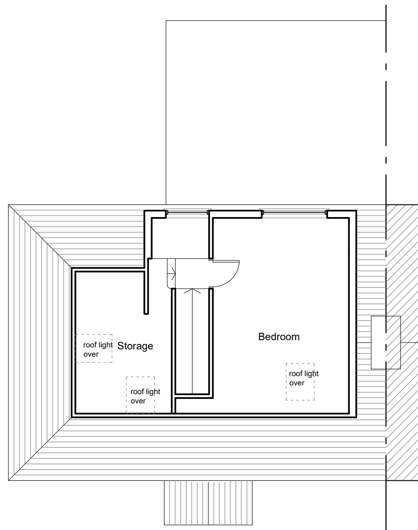
EXISTING SECOND FLOOR PLAN
