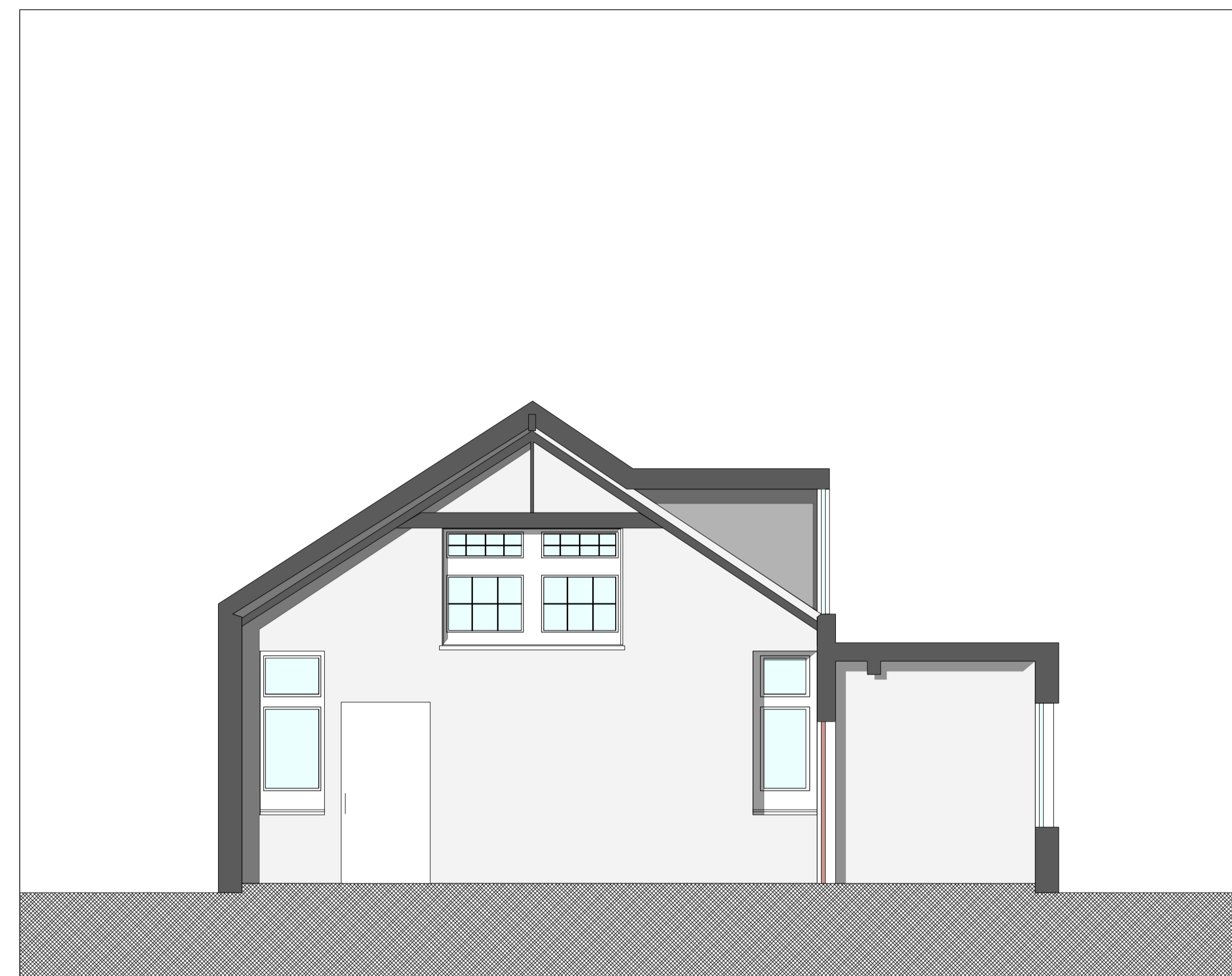
Existing Section BB 1:50
