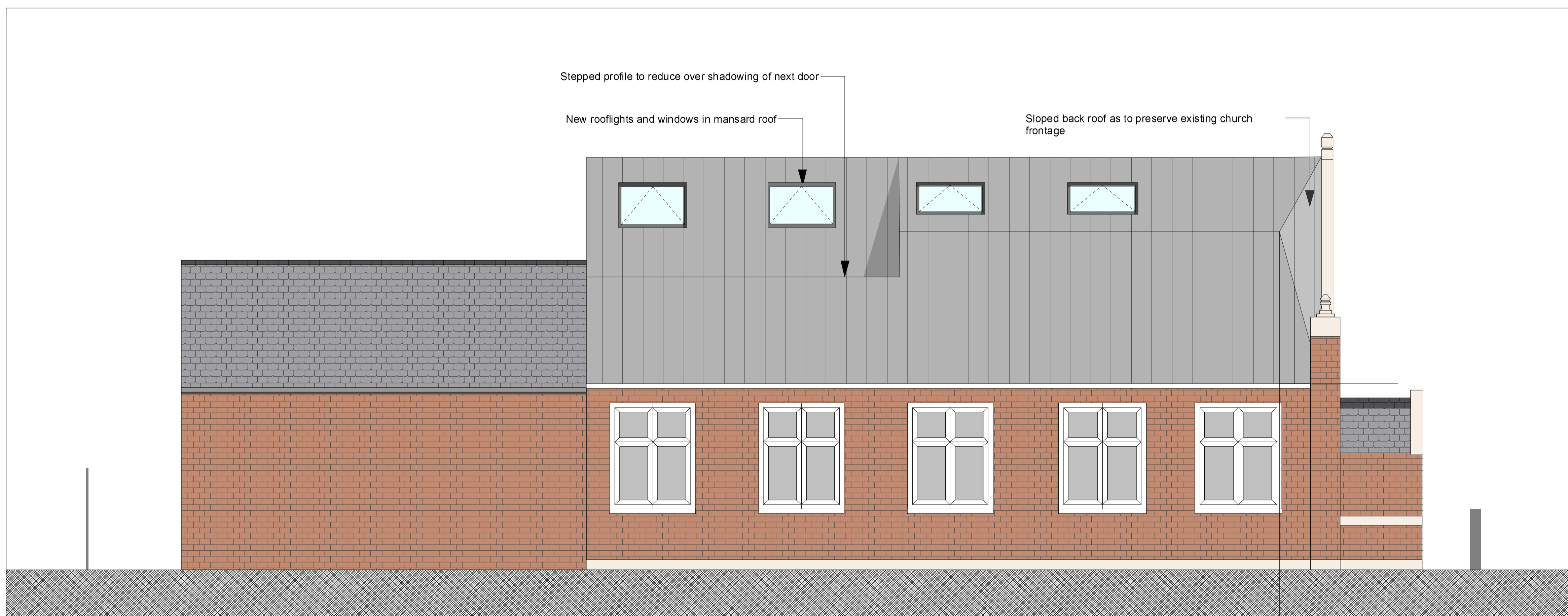
Proposed Elevation DD 1:50
