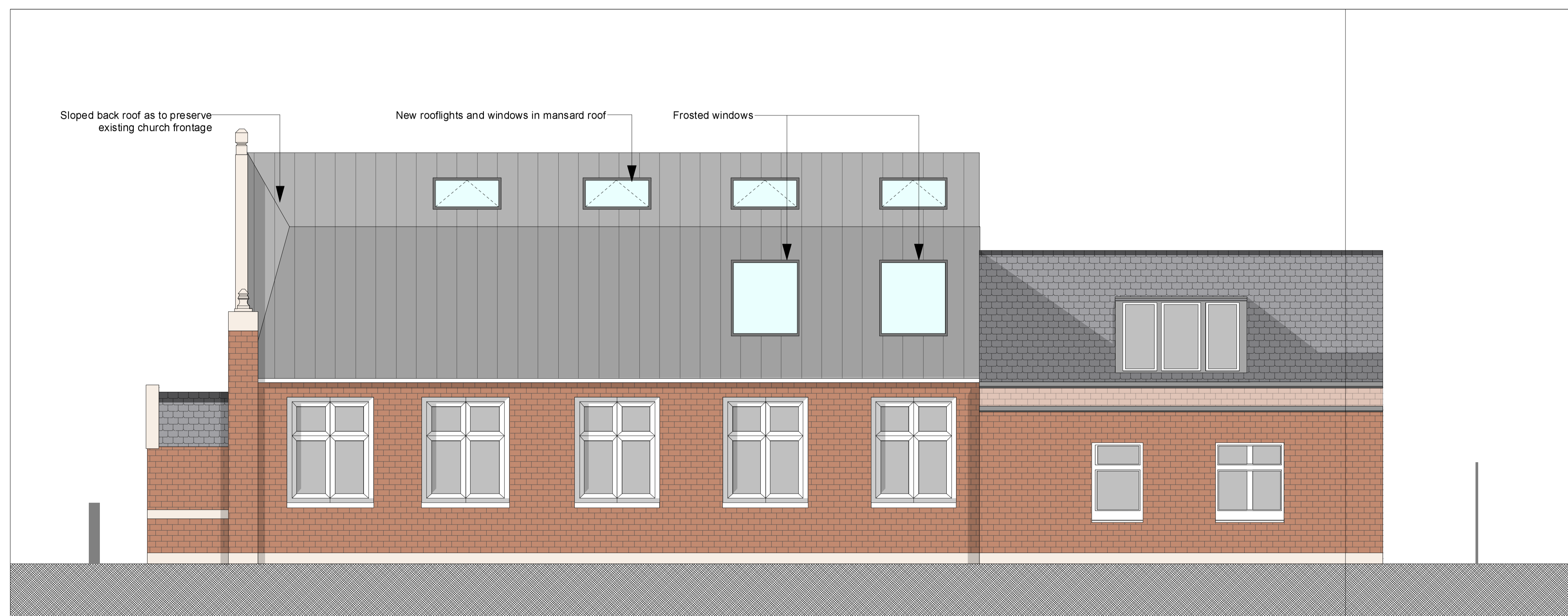
Proposed Elevation BB 1:50
