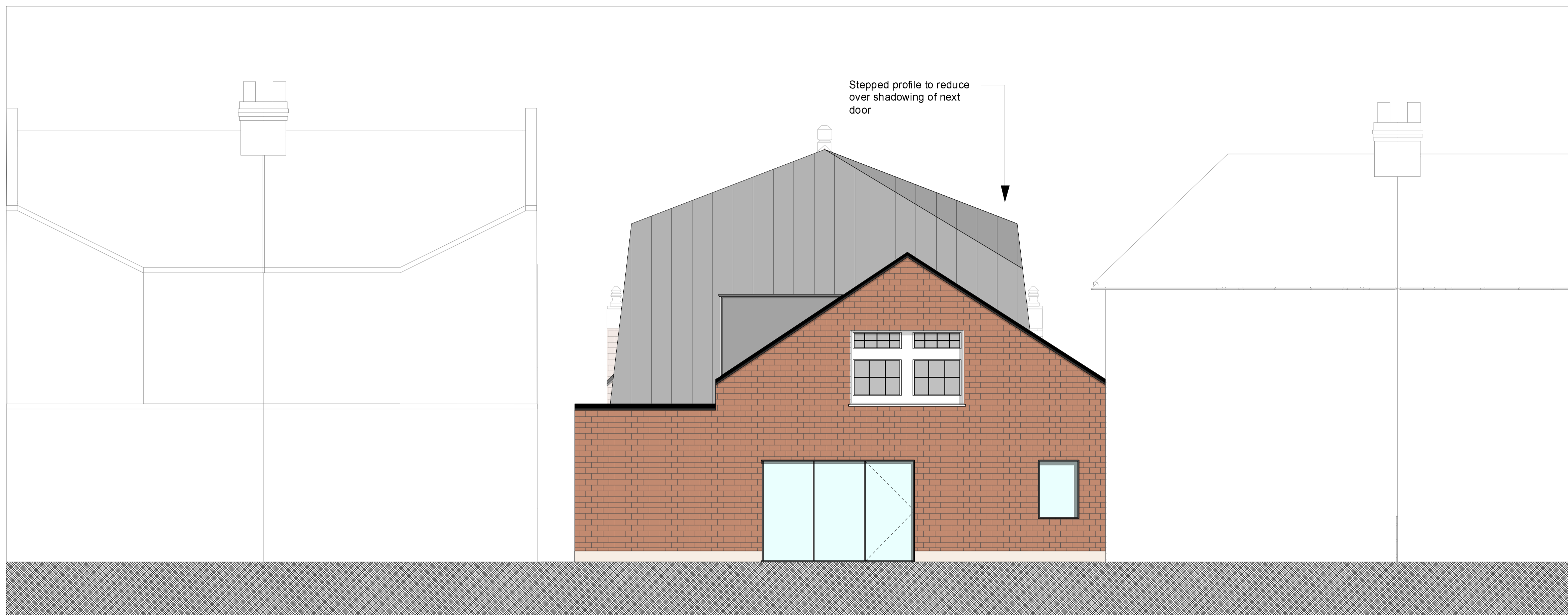
Proposed Elevation CC 1:50
