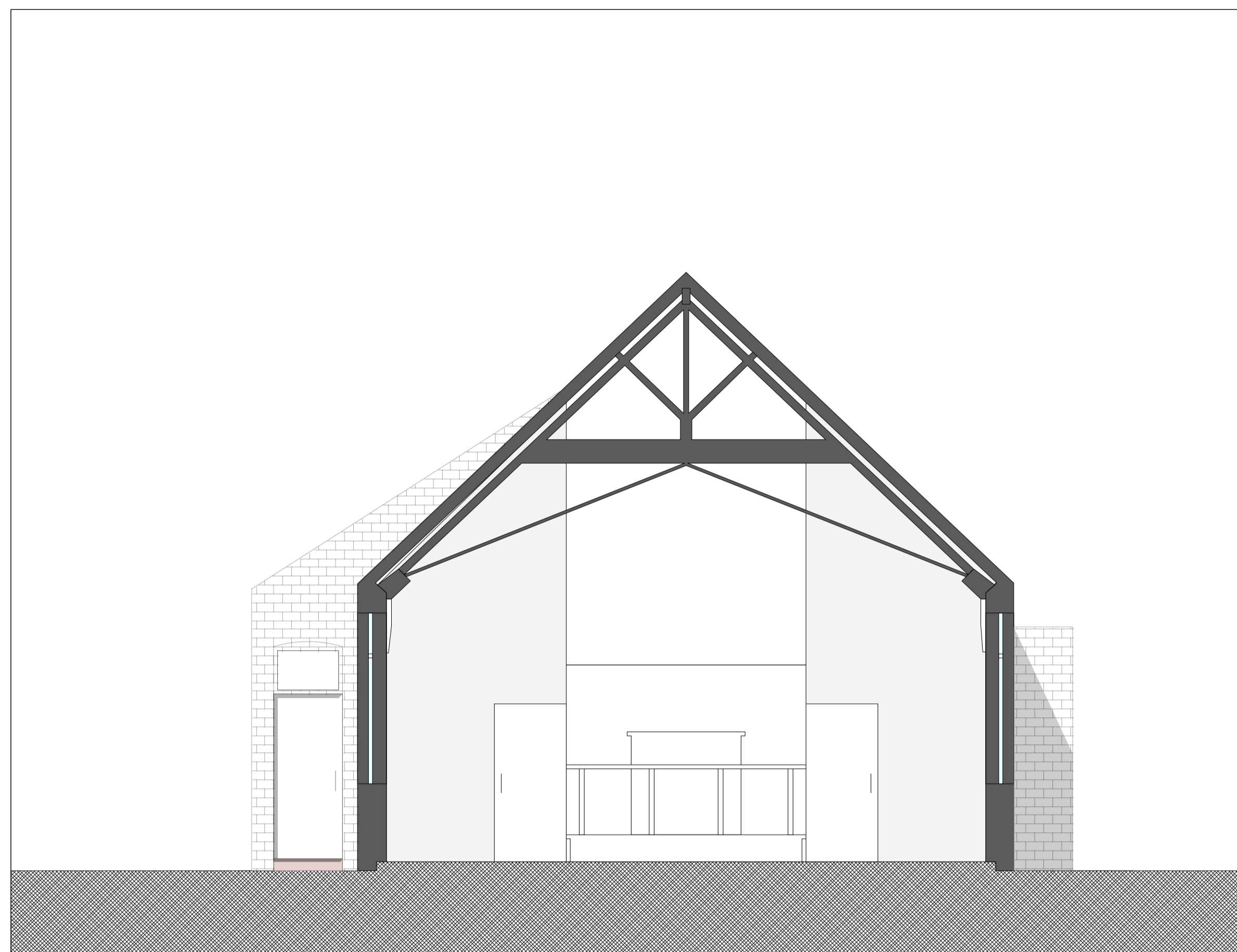
Existing Section AA 1:50
