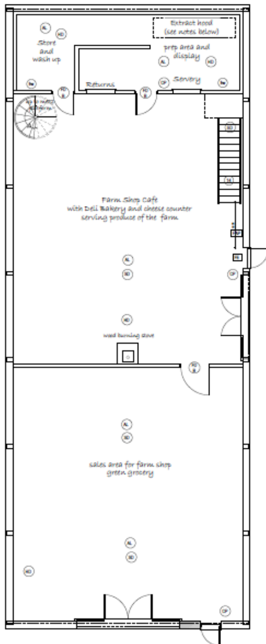
Proposed Ground Floor Plan - 1:100 Schedule and legend Project Name: Farm Shop and Cafe
