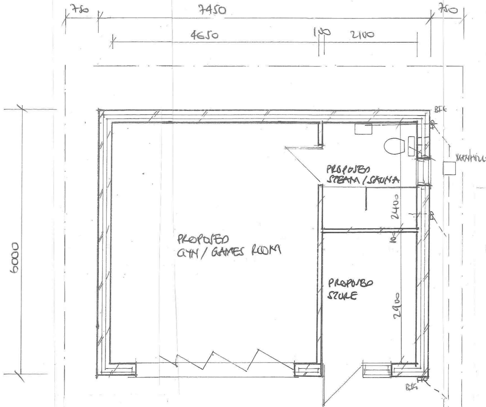
PROPOSED FLOOR PLAN LAYOUT
