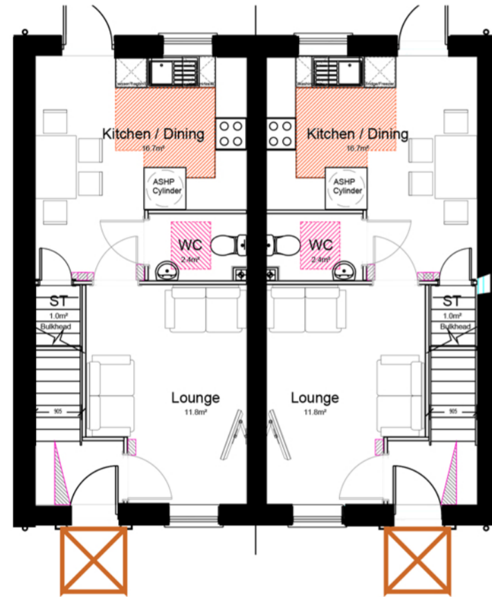
House Type 2A Total Floor Area: 70.8m 2 Ground Floor Plan
