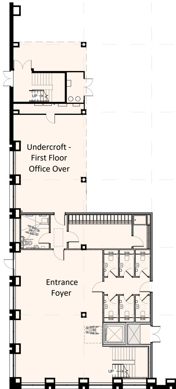
1 Unit 1 Ground Floor Core Plan 1:200
