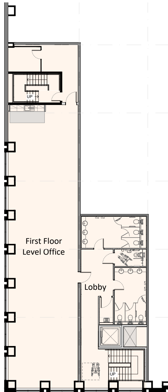
2 Unit 1 First Floor Core Plan 1:200
