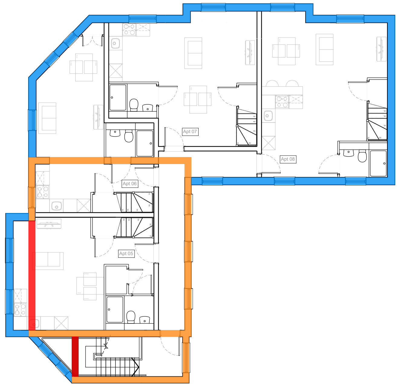
1. Ground Floor Demolition Plan
