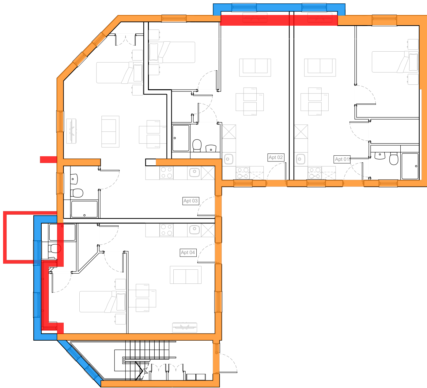
1. Ground Floor Demolition Plan
