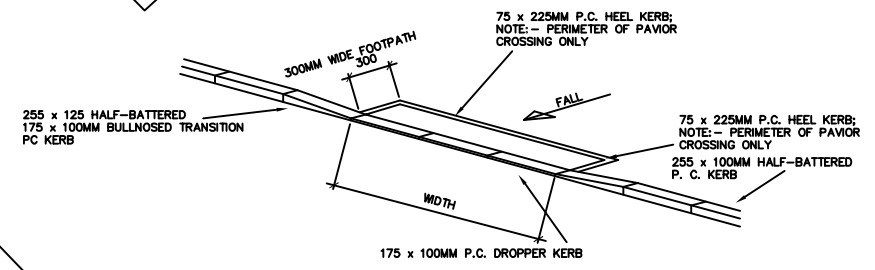
TYPICAL VEHICULAR ACCESS CROSSINGS
