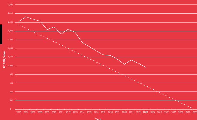
Borough-wide territorial CO 2 emissions
