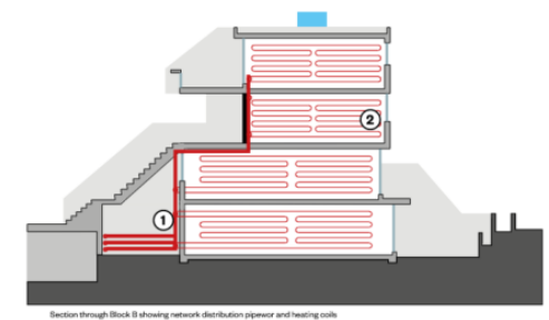
1 Estate distribution pipework 2 Heating coils
